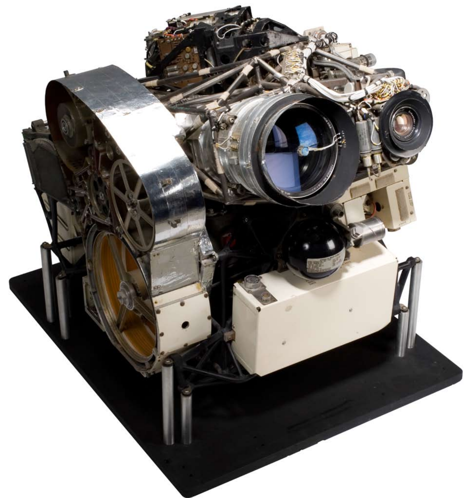
LUNAR ORBITER, 1967 Made pictures and mapped the entire surface of the moon
